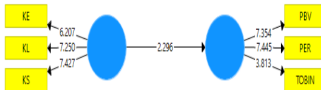
Figure 2. T-value Chart Path on the research model
