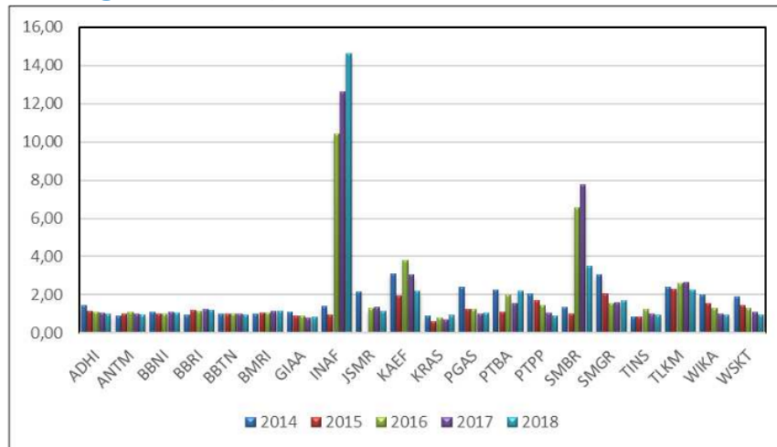
Figure 1. Tobins-Q Chart of SOEs in IDX Year 2014-2018
